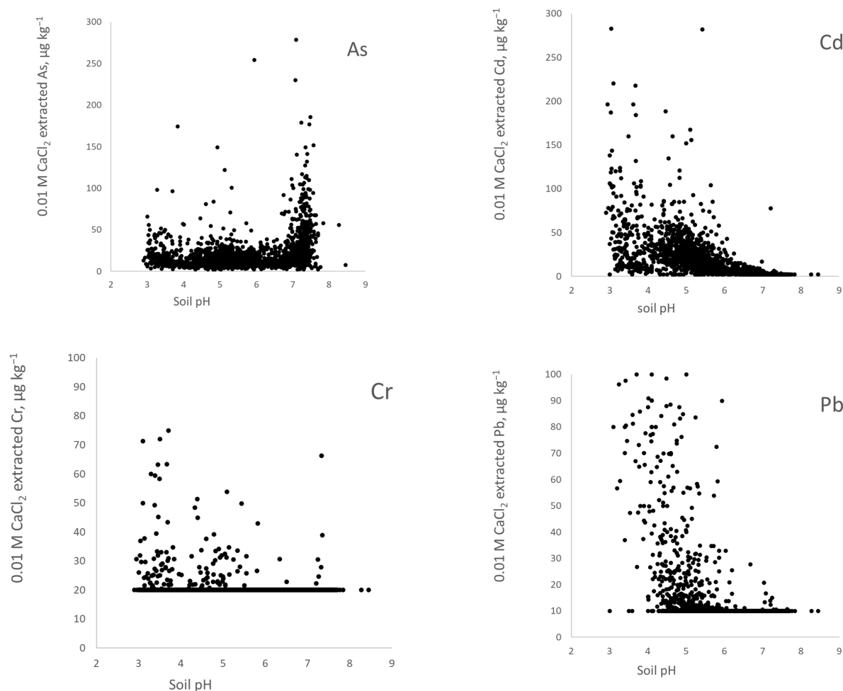
Figure 3. Relationship between soil pH—0.01 M \text{CaCl}_2 (x-axis) and 0.01 M \text{CaCl}_2 -extracted nickel (Ni), aluminum (Al), arsenic (As), cadmium (Cd), chromium (Cr), and lead (Pb) (y-axis, \mu\text{g kg}^{-1} ). Soil samples (0–25/30 cm) originate from agricultural, natural, and urban fields in Europe ( n = 1886 ).
