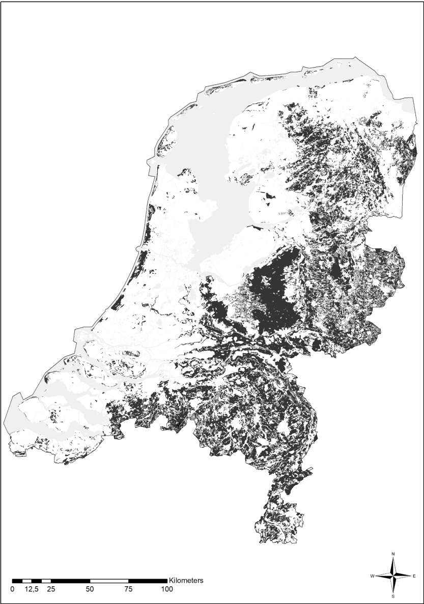
Fig. 2. Area of mineral soils, as indicated by the Soil Map of the Netherlands (1:50,000).
