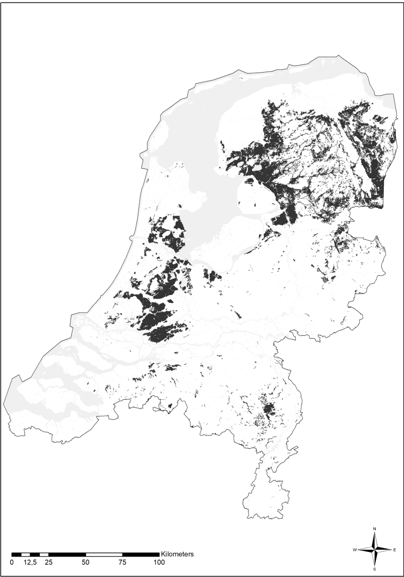
Fig. 3. Area of soils with peaty layers within 30 cm depth, as indicated by the Soil Map of the Netherlands (1:50,000).
