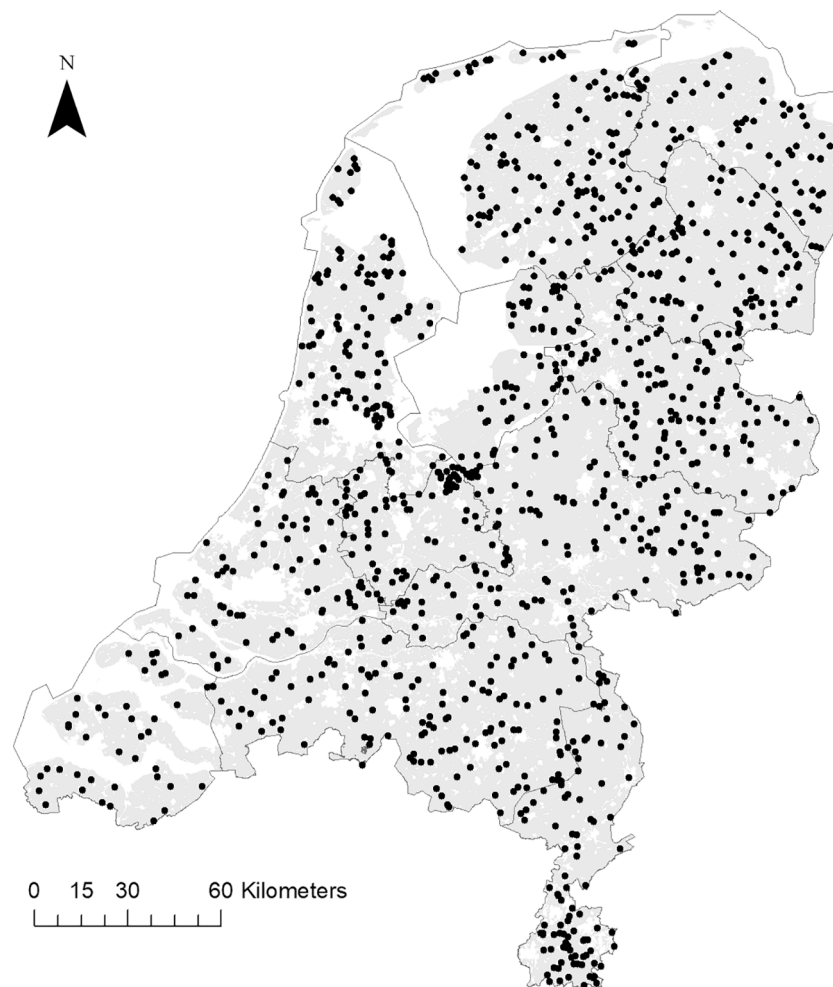
Fig. 1. Locations of the SSP (Soil Sampling Programme of the Netherlands) revisited in 2018.
